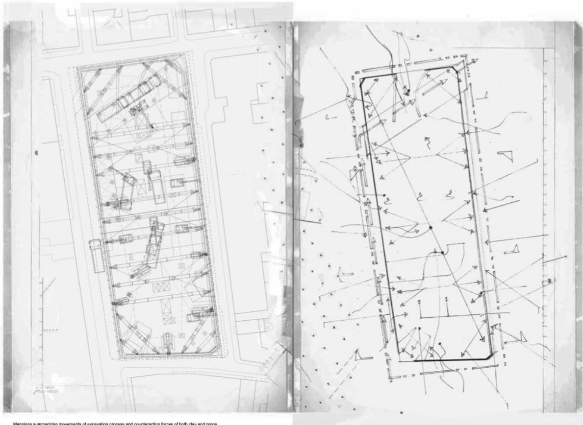
Mappings summarizing movements of excavation process and counteracting forces of both clay and props
