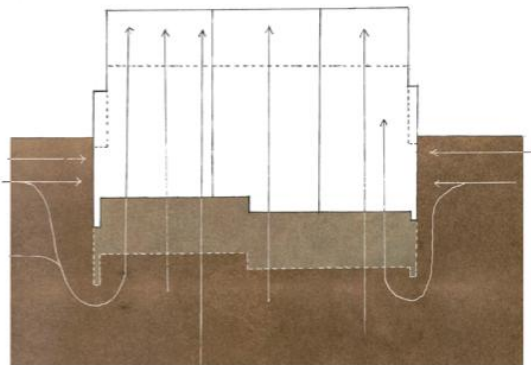
To ensure the proposed building is not pushed upwards...
