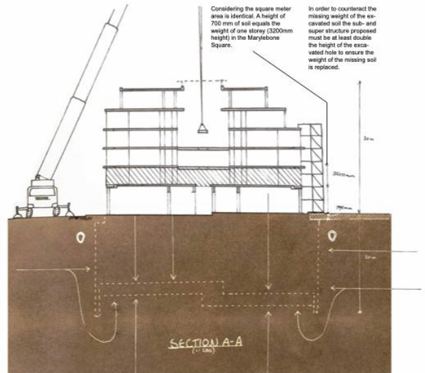
a 1200mm reinforced concrete raft is added to the building's foundation for extra weight.
