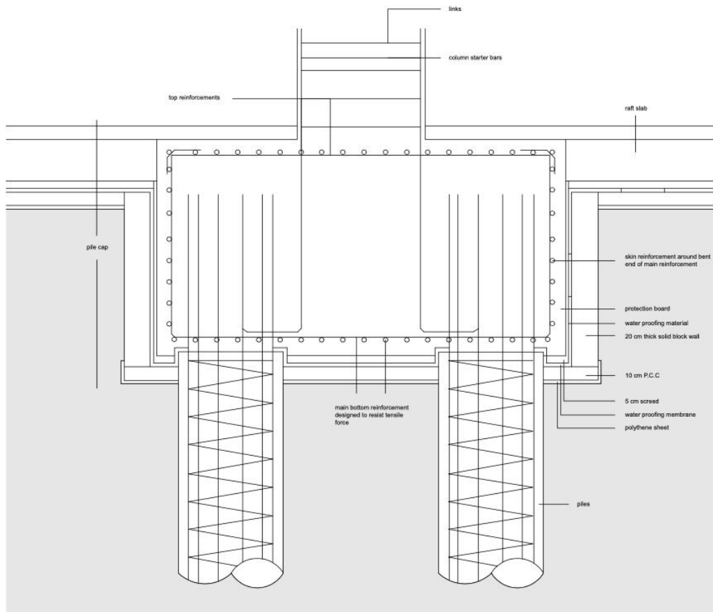
1:5 detail section of pile cap
