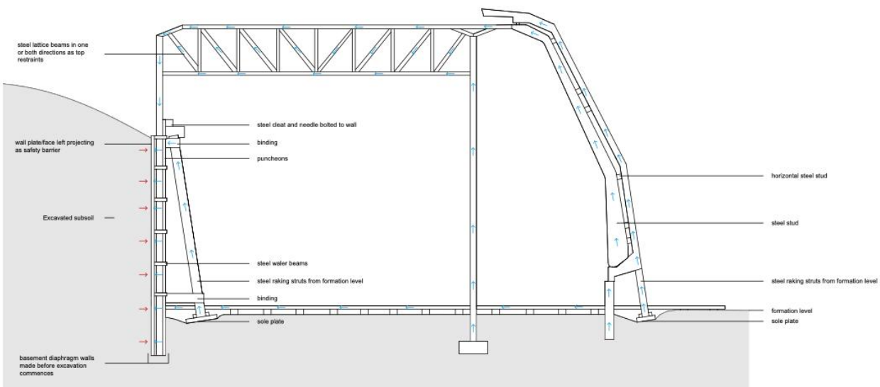
1:20 detail section of youth centre
